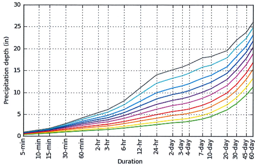
PDS-based depth-duration-frequency (DDF) curves Latitude: 39.0389°, Longitude: -76.7264°
